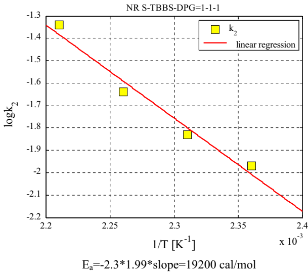
Fig. 14 NR+(S,TBBS,DPG)(1,1,1) system, k_2 constant behavior at different temperatures in the Arrhenius space and estimated activation energy
